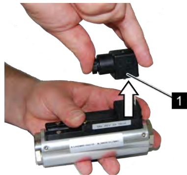
Fig. 23: Remove socket
