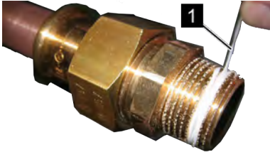
Fig. 9: Apply sealing thread
