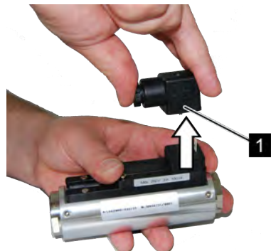
Fig. 60: Remove the female socket
