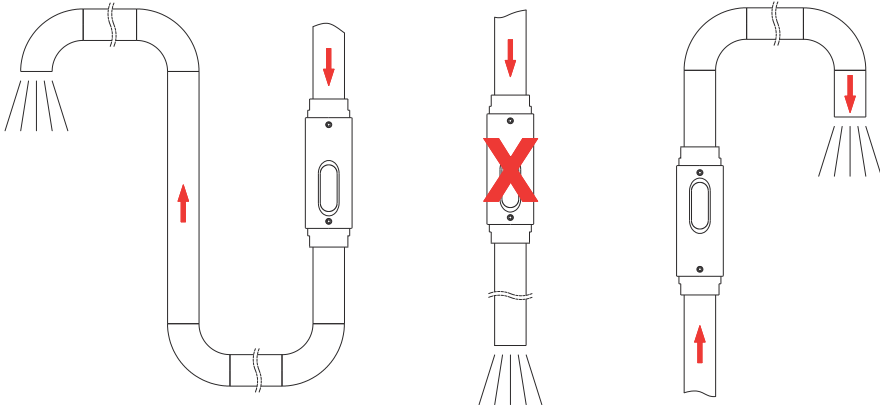
Fig. 7: Unimpeded outlet
