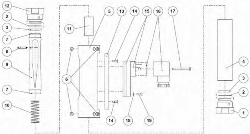
Fig. 71: Replacement parts drawing
