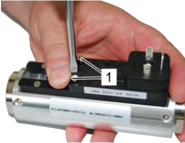
Fig. 61: Loosen set screws
