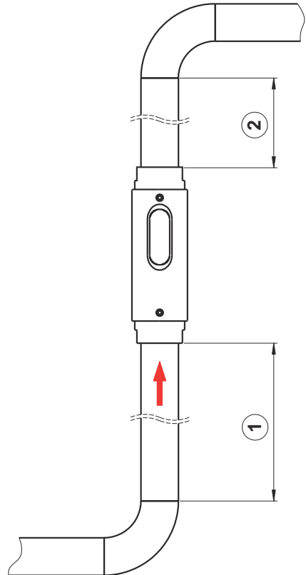
Fig. 6: Unimpeded flow section
