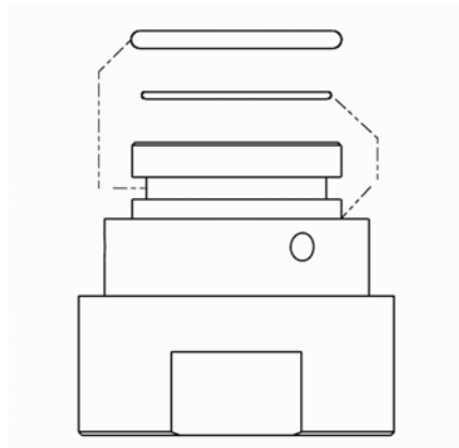
Fig. 44: Position of O-rings
