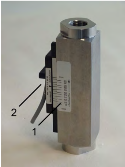
Fig. 1: DUM flow monitor
