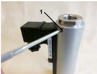
Fig. 36: Remove the process connection (outlet)
