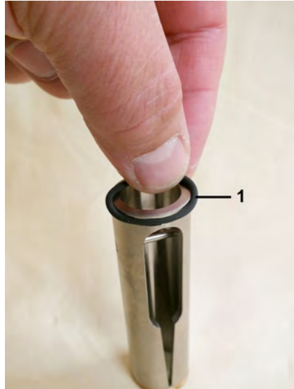
Fig. 44: O-ring (centering the slot nozzle)
