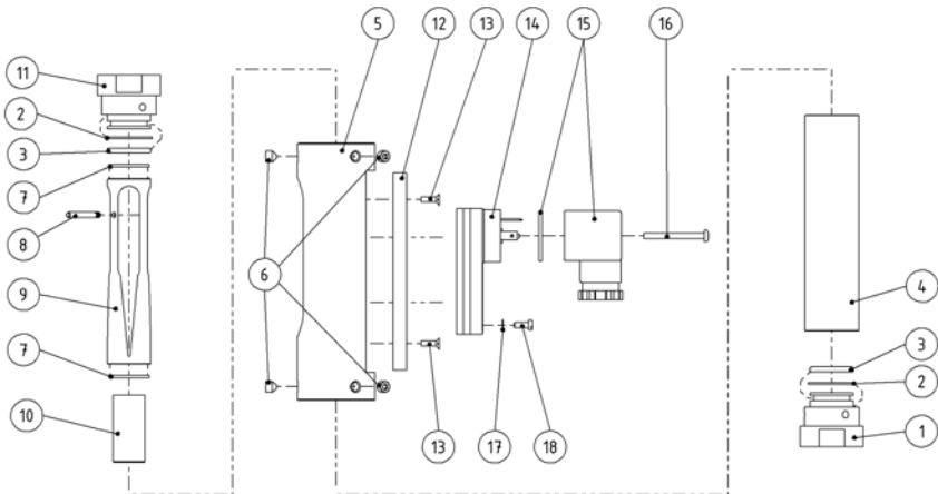
Fig. 68: Replacement parts drawing
