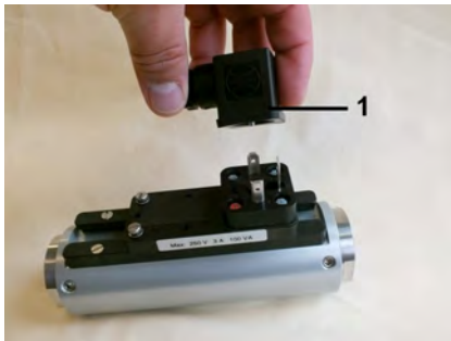
Fig. 58: Remove the female socket
