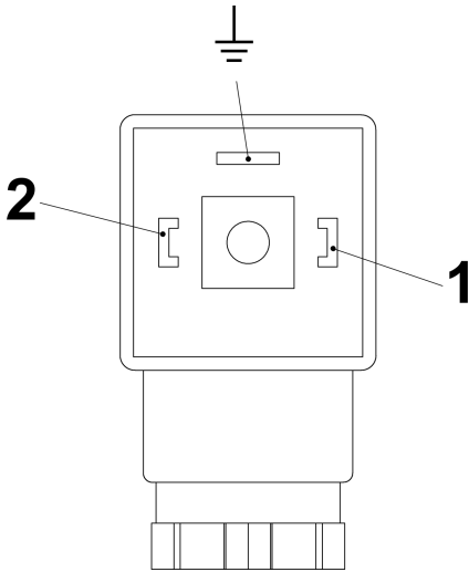
Fig. 25: Pin assignment, plug socket, normally-open contact (SG-30 with connector in compliance with EN175301-803)
