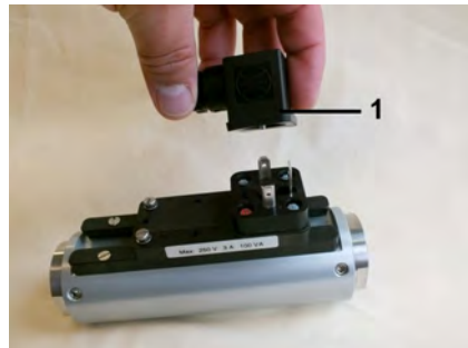
Fig. 22: Remove socket
