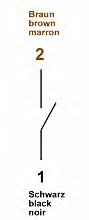
Fig. 20: Switch position under no-flow condition
