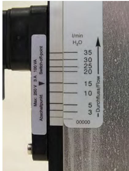
Fig. 4: DWM switch point adjustment scale
