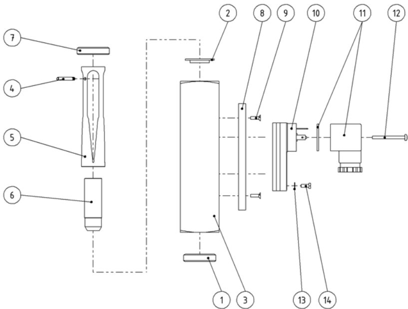
Fig. 68: Type DWM-35 and DWM-50 (G1")
