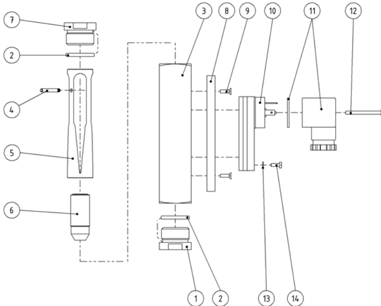
Fig. 66: Type DWM-1,5 through DWM-18
