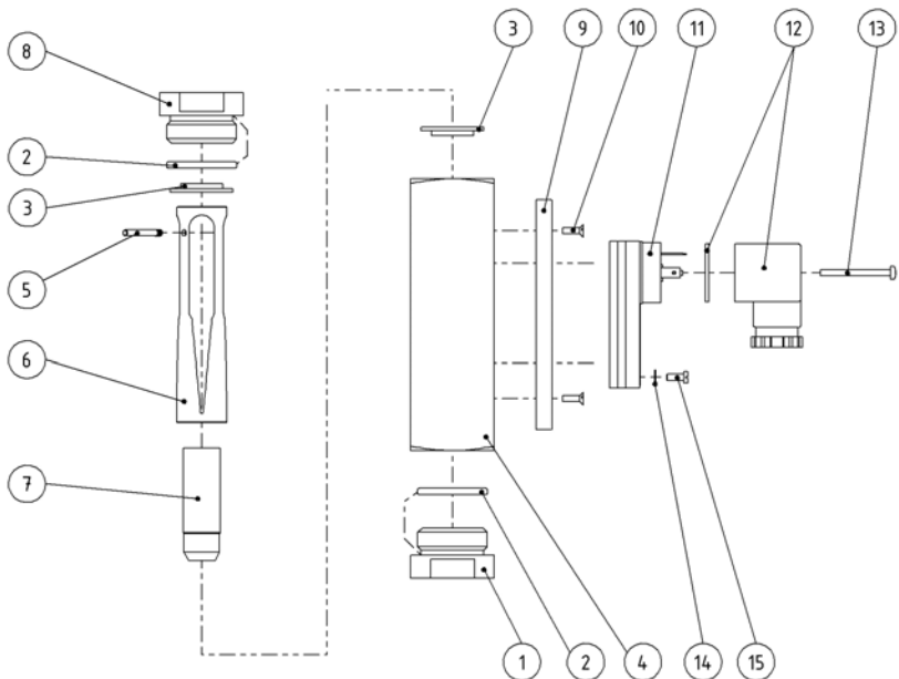
Fig. 67: Type DWM-35 and DWM-50 (G3/4")
