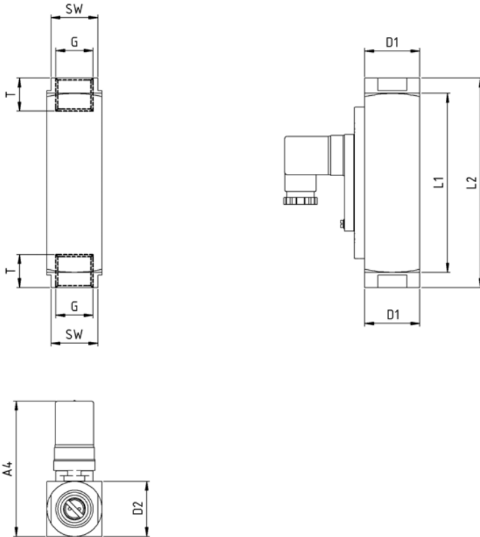
Fig. 64: Type DWM-35 thru DWM-50 ( G\frac{3}{4} "
