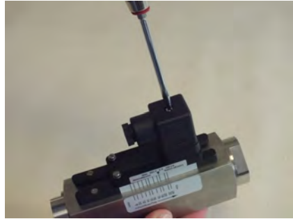
Fig. 53: Loosen female socket
