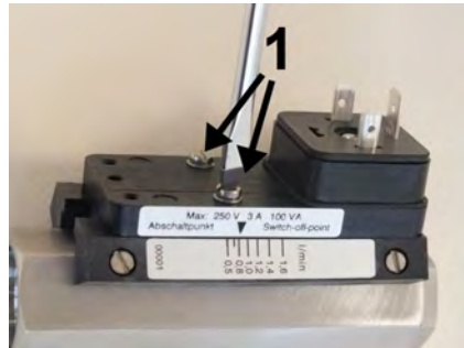
Fig. 56: Loosen set screws
