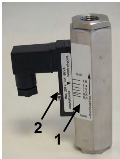
Fig. 1: DKM-2 flow monitor
