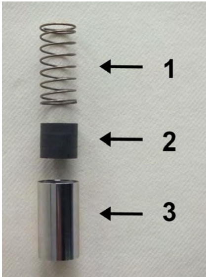
Fig. 48: Inner parts
