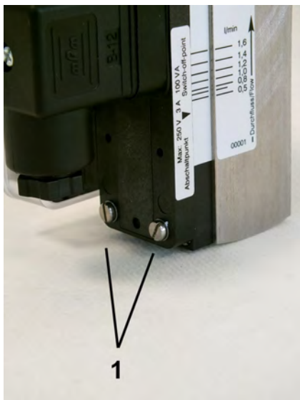
Fig. 34: Loosen set screws
