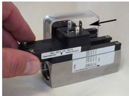
Fig. 71: Remove switch contact from guide rails
