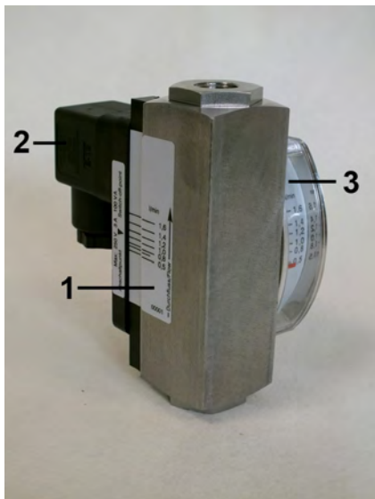
Fig. 1: DKM/A-2 30x70 flow monitor
