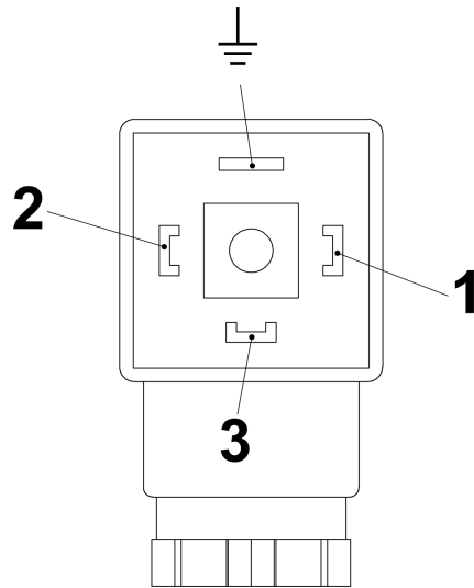
Fig. 28: Pin assignment, plug socket, Change-over contact (Form 30x70)
