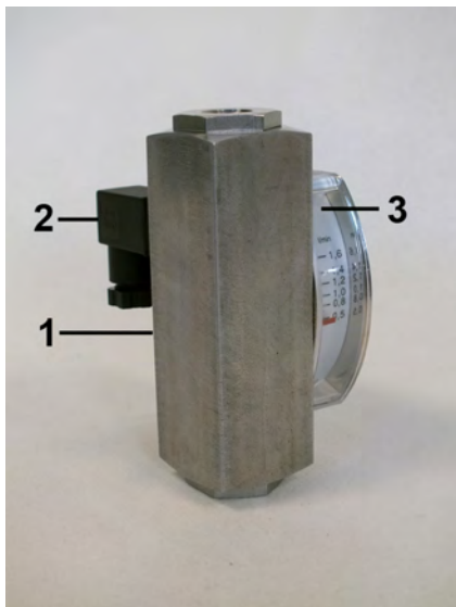
Fig. 1: DKM/A-2 flow monitor
