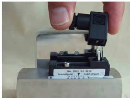
Fig. 23: Remove socket
