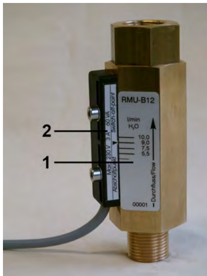
Fig. 1: RMU-B flow monitor
