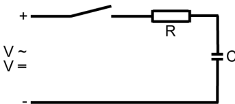
Fig. 20: Protective measure against capacitive loads
