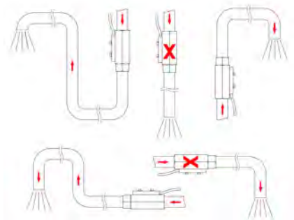
Fig. 7: Unimpeded outlet
