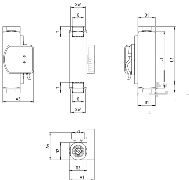
Fig. 3: Type DWM/A-L18 through DWM/A-L50 ( G^{3/4} ")
