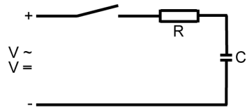
Fig. 30: Protective measure against capacitive loads
