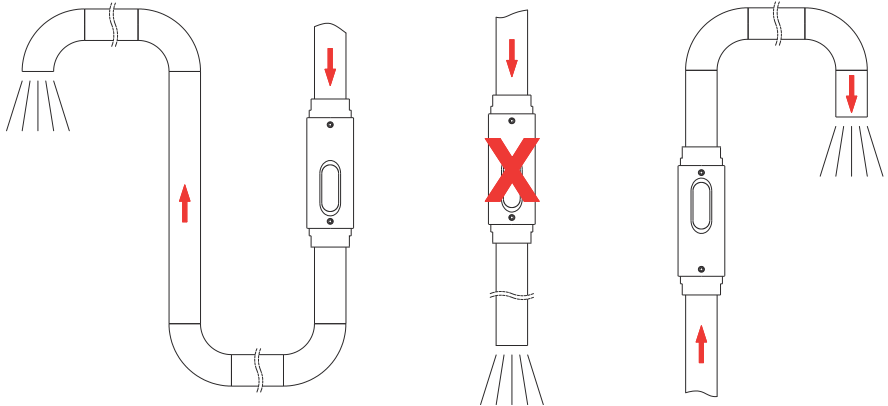
Fig. 7: Unimpeded outlet
