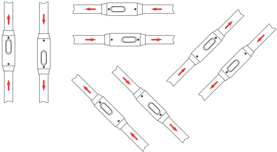
Fig. 5: Installation position/direction of flow
