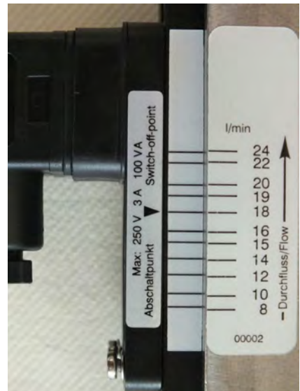
Fig. 4: Switch point adjustment scale DKM/A-1
