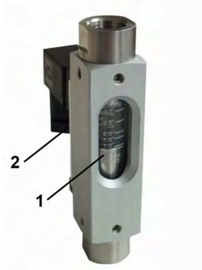
Fig. 1: Flow monitor RVO/U-4
